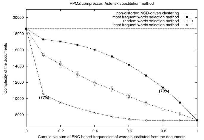
(b) UCI-KDD data set. Upper bound estimation of the documents complexity.
