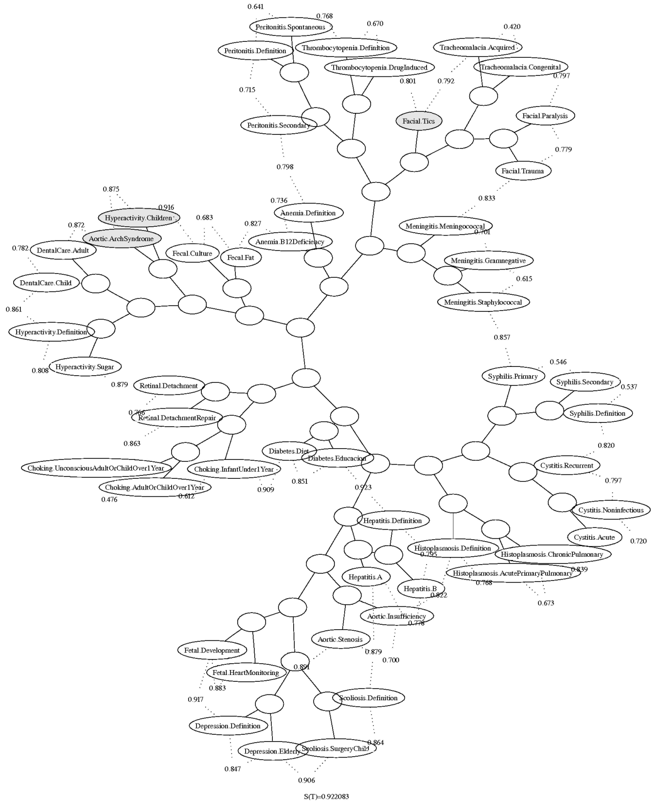
Fig. 10. Example of dendrogram for the extended MedlinePlus repository. The numbers in the image represent the NCD average between two nodes. The dendrogram corresponds to the figure 9(b), in particular, it corresponds to the 0.7 cumulative sum of frequencies for the most frequent words selection method graph. The documents which have not been correctly clustered are highlighted in gray. Note that only three documents have not been correctly clustered: Facialtics , Aorticarchsyndrome and Hyperactivityandchildren .
