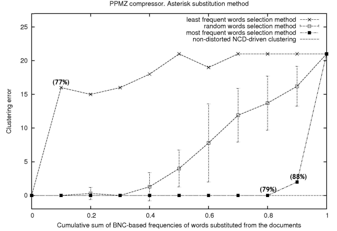
(a) UCI-KDD data set. Clustering error.
