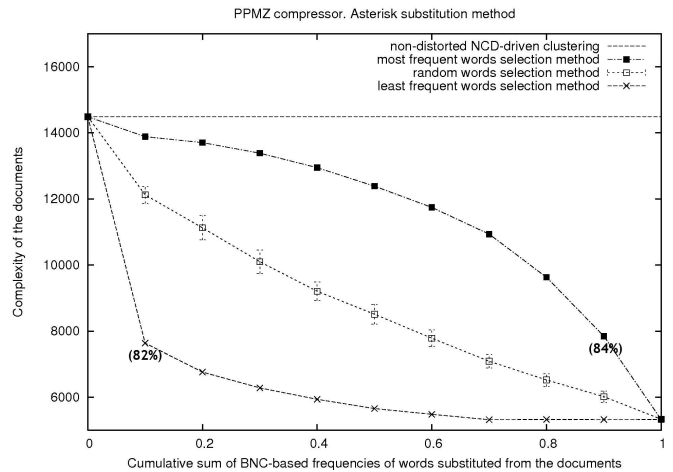
(b) IMDB data set. Upper bound estimation of the documents complexity.
