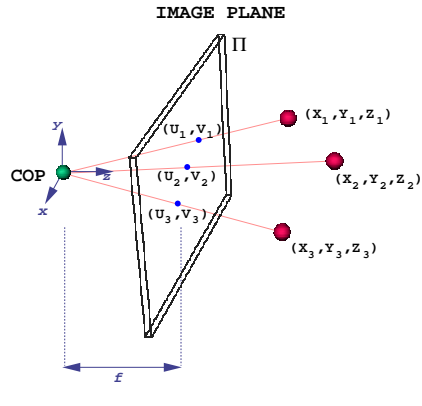
Fig. 3. Perspective Projection
