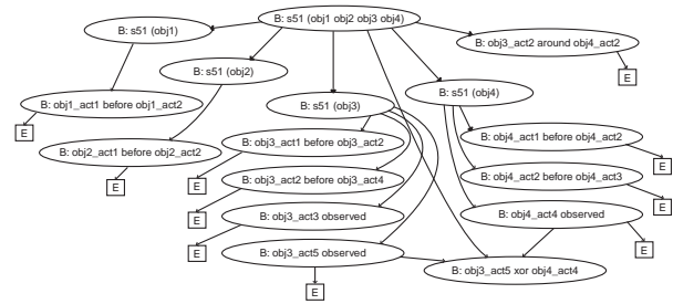
Figure 6: The s51 multi-agent recognition network.
