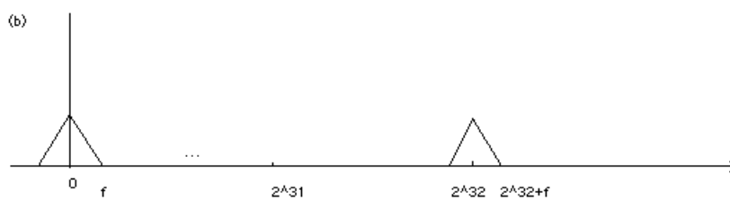
(a) -- Spectrum of signal evenly sampled at 8kHz (b) -- Spectrum of signal unevenly sampled with T = 2^{32}
