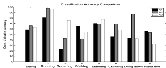
Figure 1. K-fold cross validation accuracy comparison using a single accelerometer.
