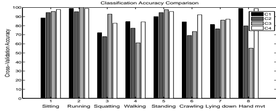
Figure 2. K-fold cross validation accuracy comparison for the four different configurations of accelerometer placement.
